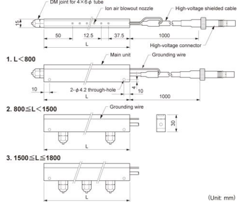
The position of the air joint is different depending on length.
